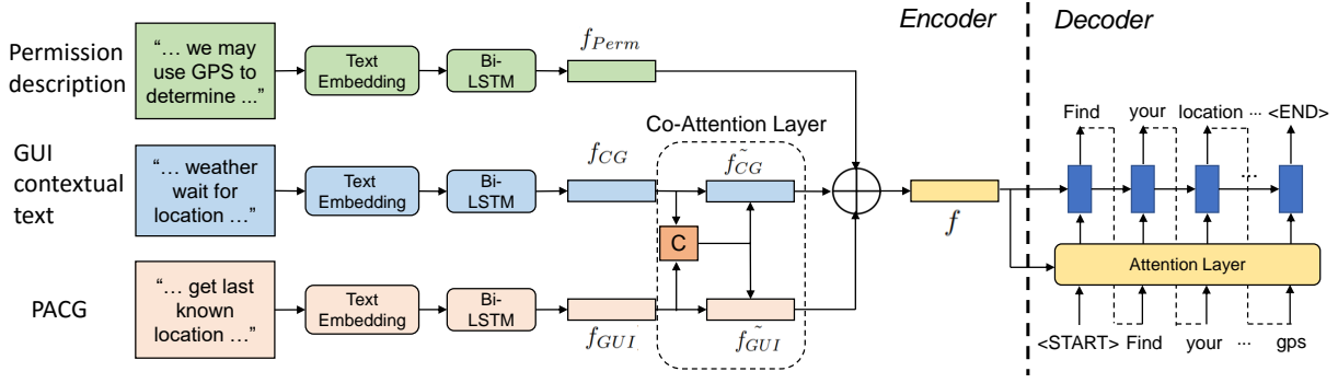
Figure 4: Overview of the behavior-description learning model.
