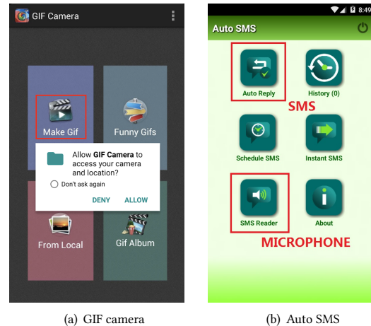
Figure 1: Example apps' GUIs: (a) permission request; (b) GUI context for SMS and microphone permissions.
