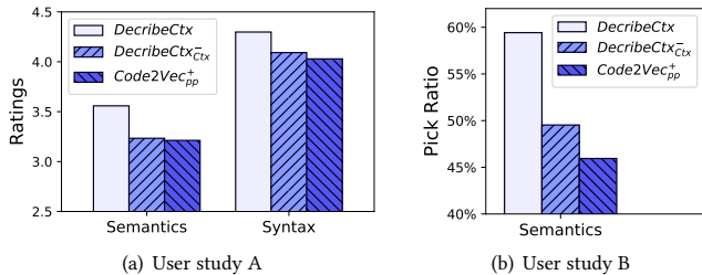
Figure 5: User ratings for the synthesized descriptions of different approaches. The proposed DESCRIBECTX is better than the two competitors in both user studies.
